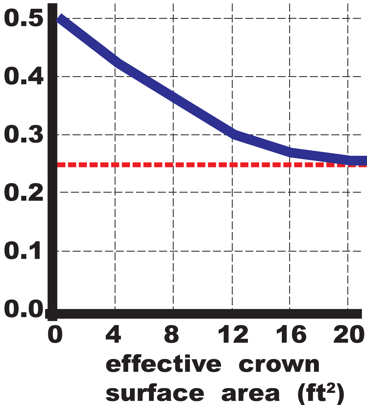
Figure 17: Ratio of tree transpiration to pan evaporation (pan factor or pan coefficient). Pan factors are not less than 0.25 for trees with larger than 20 ft 2 of effective crown surface area. (after Lindsey & Bassuk, 1992)
