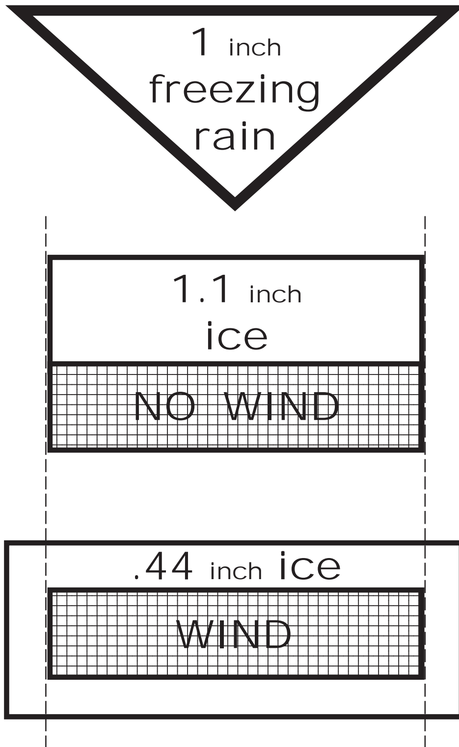
Figure 9: Freezing rain striking flat plates of equal size, and ice accumulation with wind (>4.5 mph) and without wind. (same depth of freezing rain intercepted & uniform dry growth form ice) (Jones 1996) (Yip 1995)
