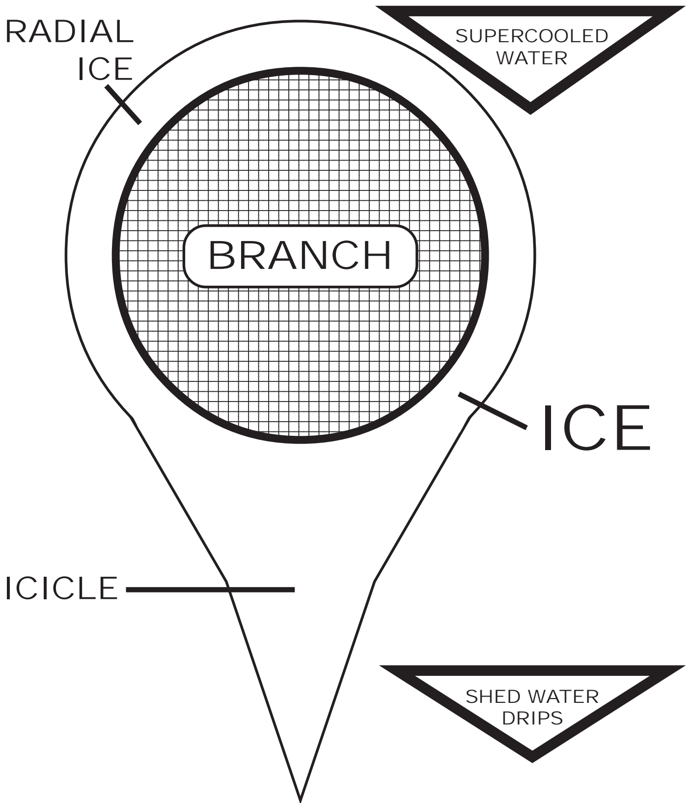
Figure 2: Glaze ice on tree branch cross-section (with surface below freezing) in freezing rain. (after Makkonen 1998)
