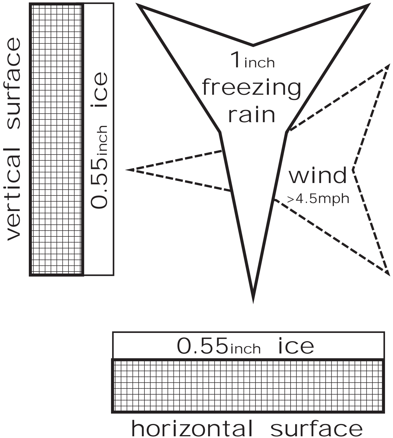
Figure 8: Freezing precipitation interception and ice accumulation on horizontal and vertical surfaces in wind. (uniform dry growth form ice) (Jones 1996) (Yip 1995)
