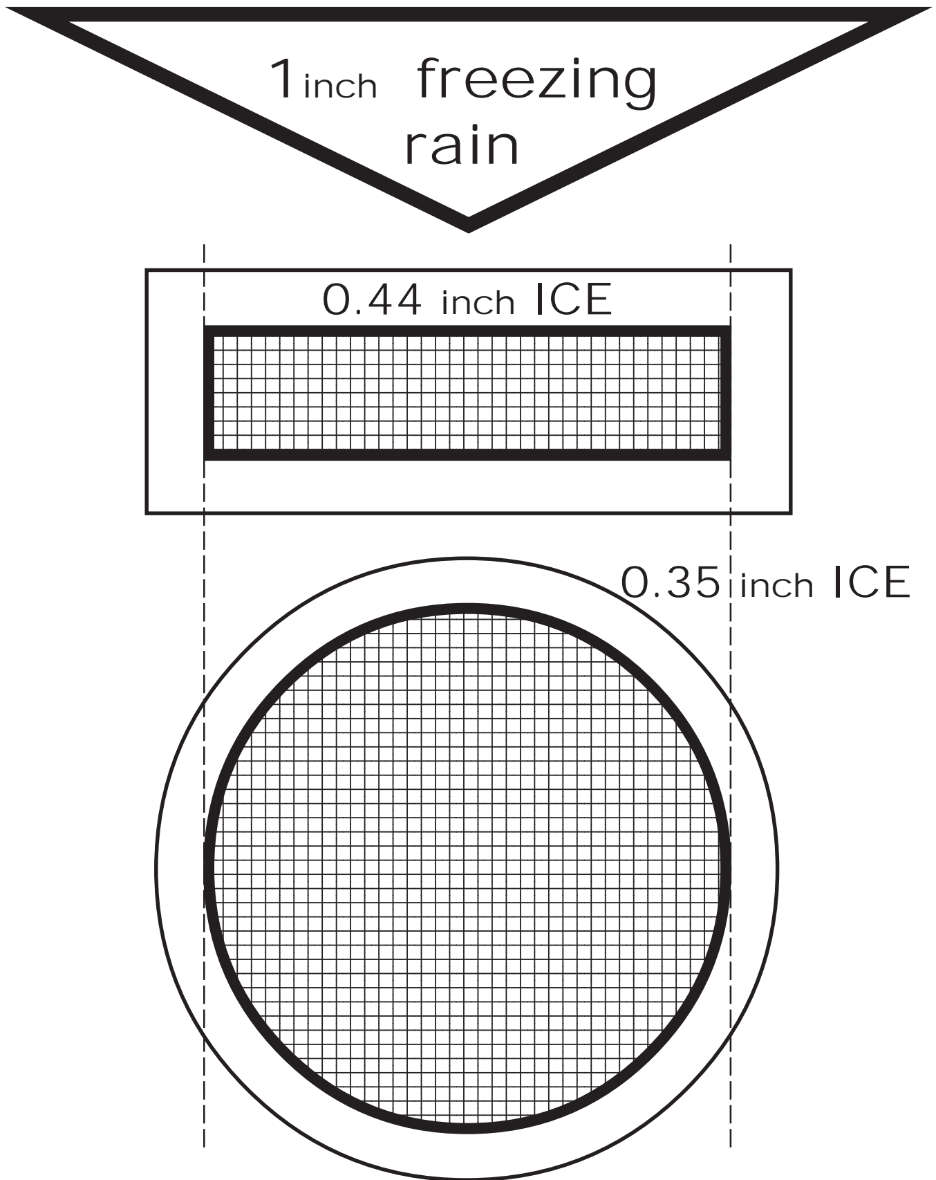
Figure 10: Freezing rain impacts a 4 inch flat surface, and a 4 inch diameter branch in wind (>4.5 mph). (Jones 1996) (Yip 1995)
