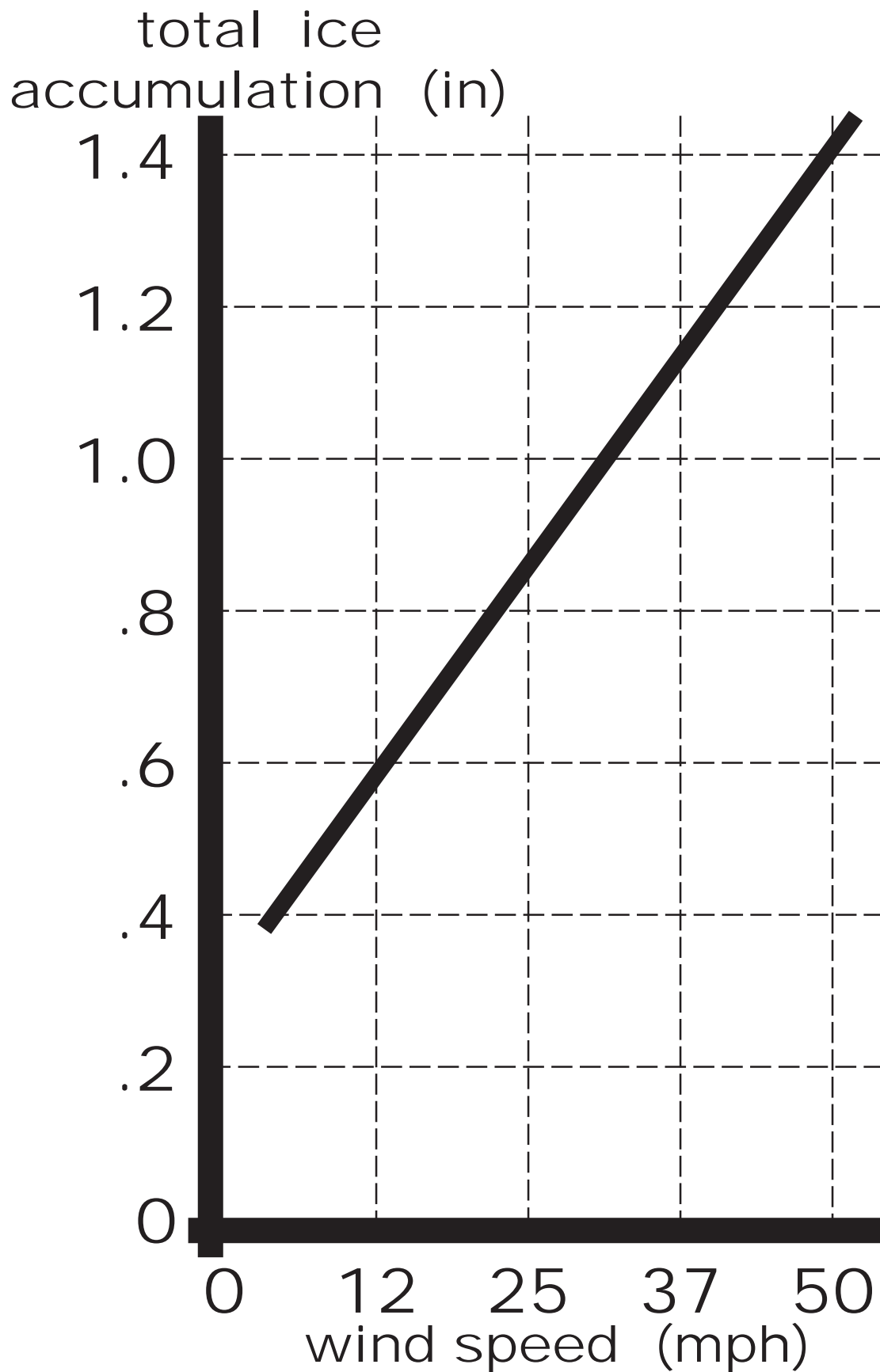
Figure 12: Impact of wind speed (mph) on ice accumulation (in.) in ice storms. (derived from Yip 1995)
