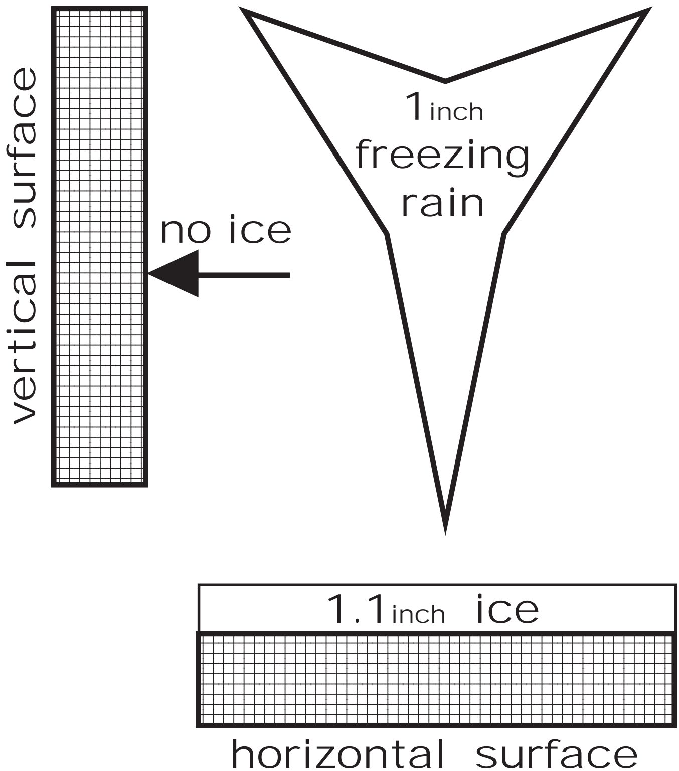
Figure 7: Freezing precipitation interception and ice accumulation on horizontal and vertical surfaces with no wind. (uniform dry growth form ice) (Jones 1996) (Yip 1995)
