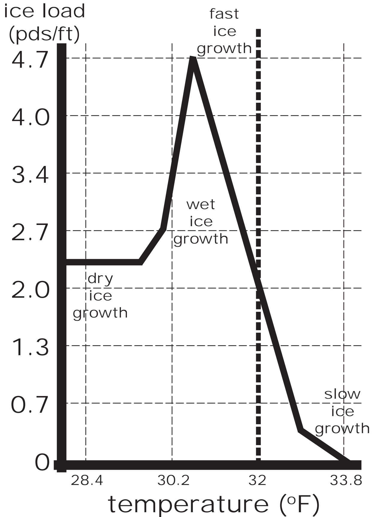
Figure 5: Temperature impacts on branch ice loads. (derived from Makkonen 1998)
