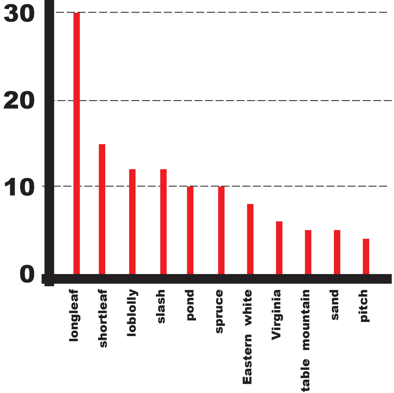
Figure 17: Expected years to sexual maturity / female cone production for Georgia pines under normal conditions.
