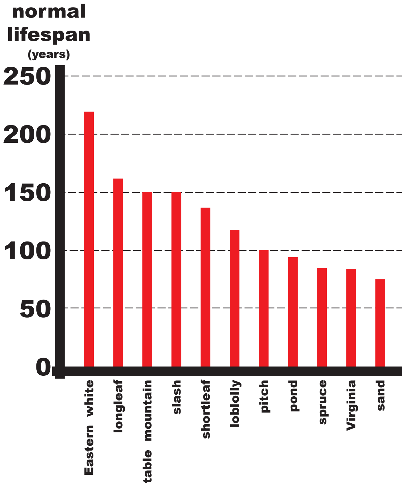
Figure 24: Normal / average lifespans (in years) of Georgia pines under non-extreme, low stress conditions.
