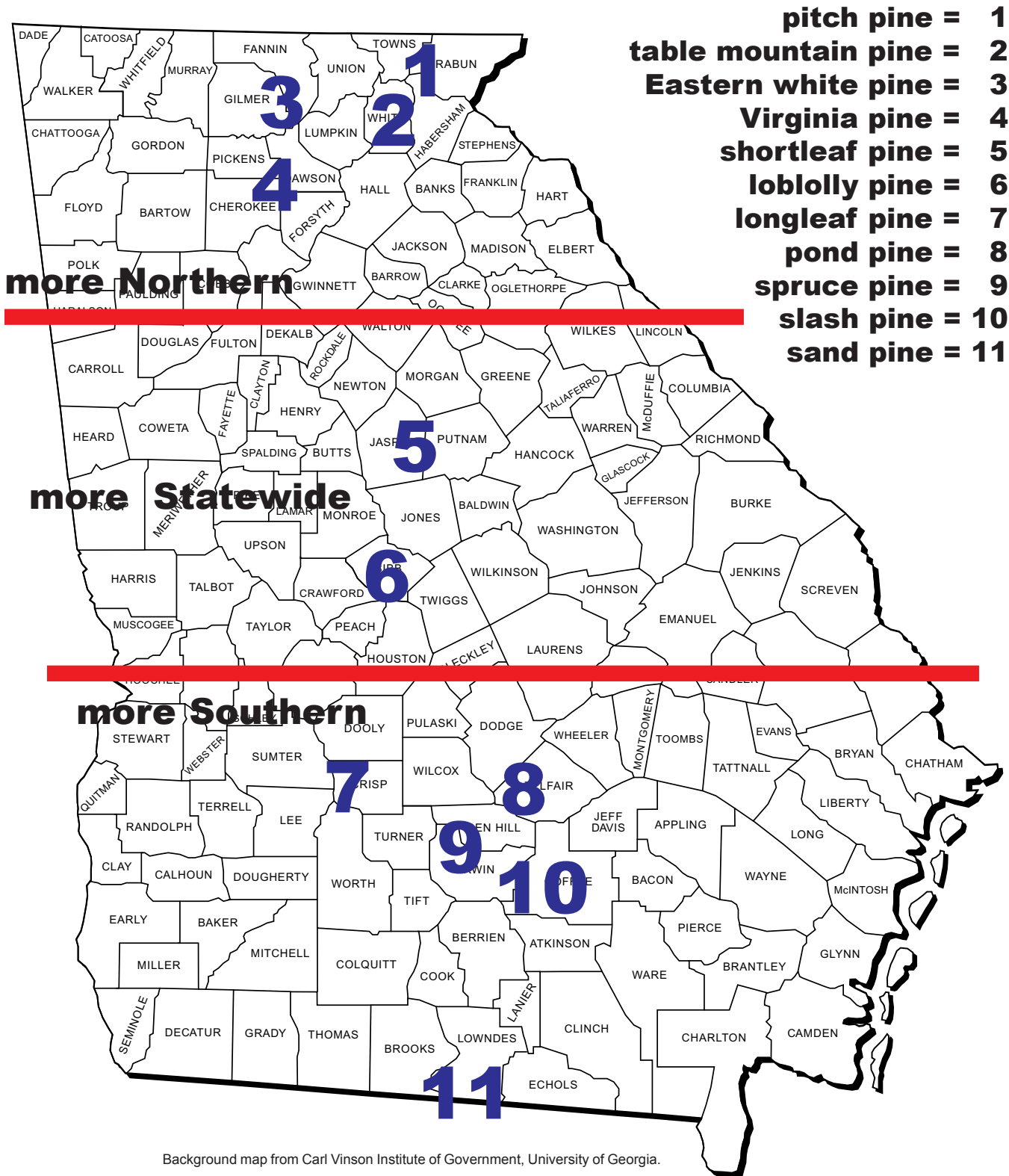
Figure 4: Center of Georgia pines native ranges. Numbers represent common names of pines and are placed in an idealized center of their growth range within Georgia.
